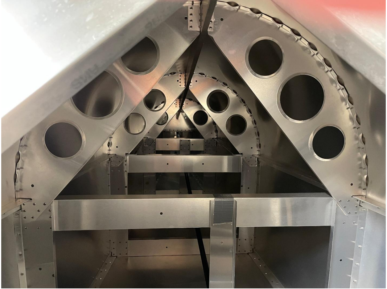
Fuselage Interior
