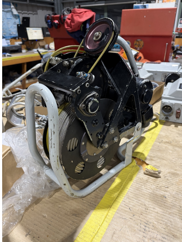
Breeze rescue hoist cable drum/mechanism - detailed view.
